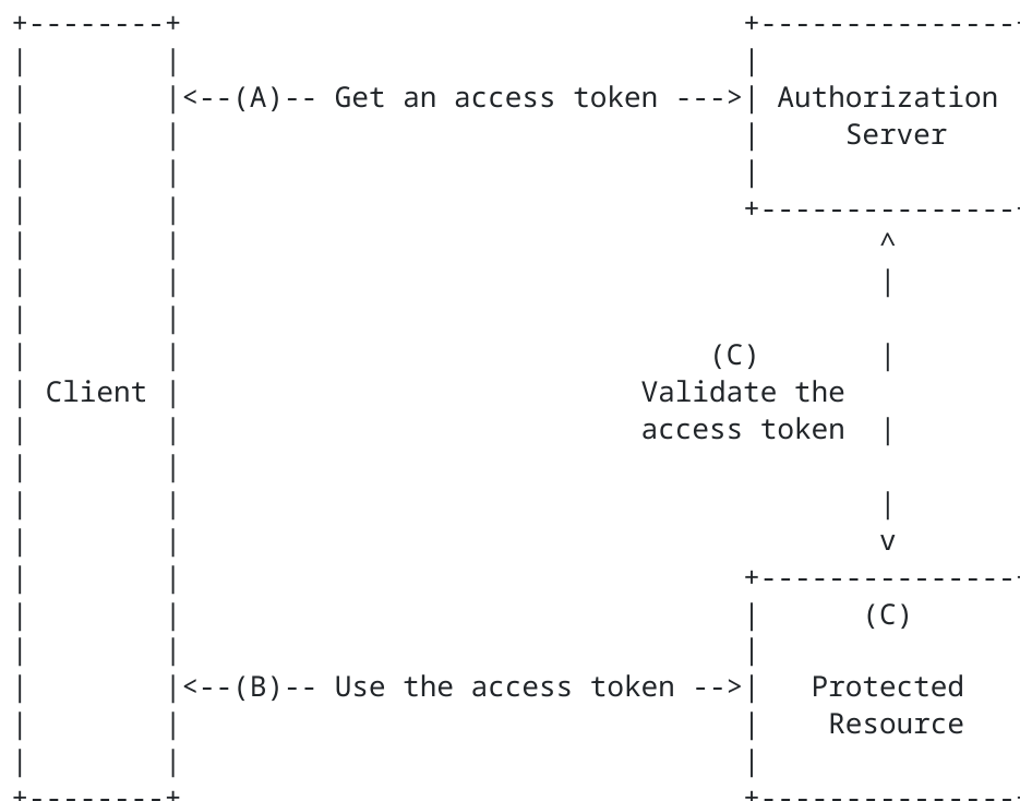
Figure 1: Abstract OAuth 2.0 Protocol Flow
