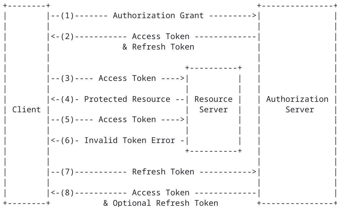
Figure 2: Refreshing an Expired Access Token
