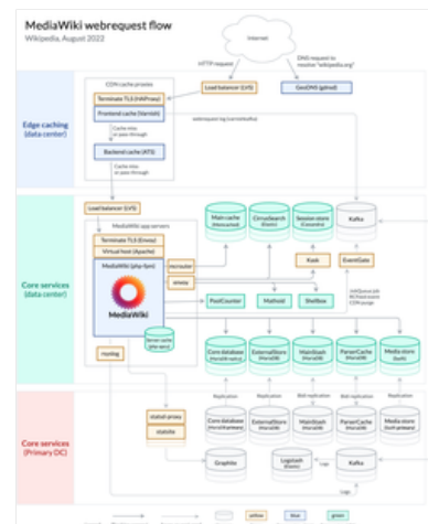
Overview of system architecture as of August 2022
