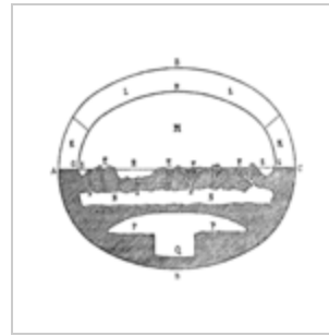
Cosmography of Old Testament (Schiaparelli).png 2,430 × 2,146; 79 KB
