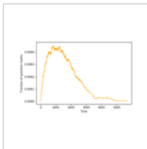
Fraction of nodes with question mark state.png 408 × 266; 13 KB
