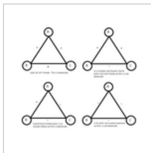
Structural Balance Triads.png 655 × 565; 19 KB
